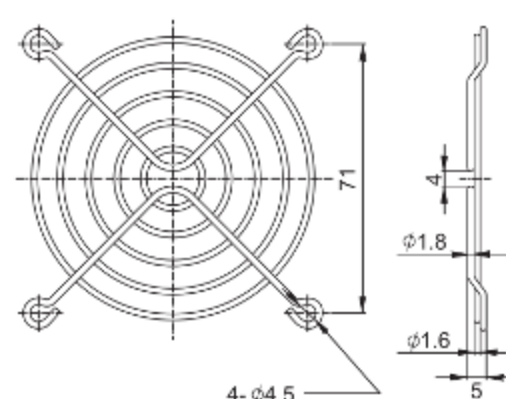
FG-08 For 80mm Fan
