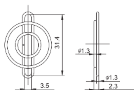
FG-02 For 25mm Fan
