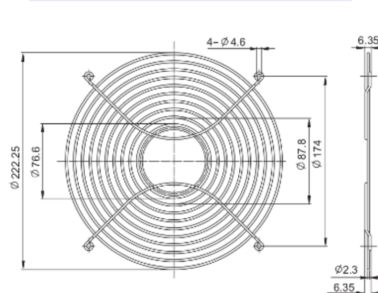
FG-25 For 254mm Fan
